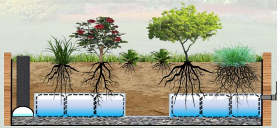
保水栽培床 Self Watering Wicking Beds
